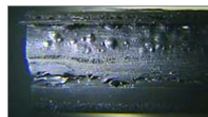
O-ring exposed to rapid depressurization
