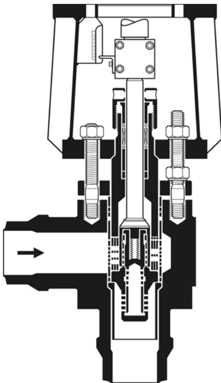
Control valve ZK 213-E.../... size 1 and 2, 6-stages
