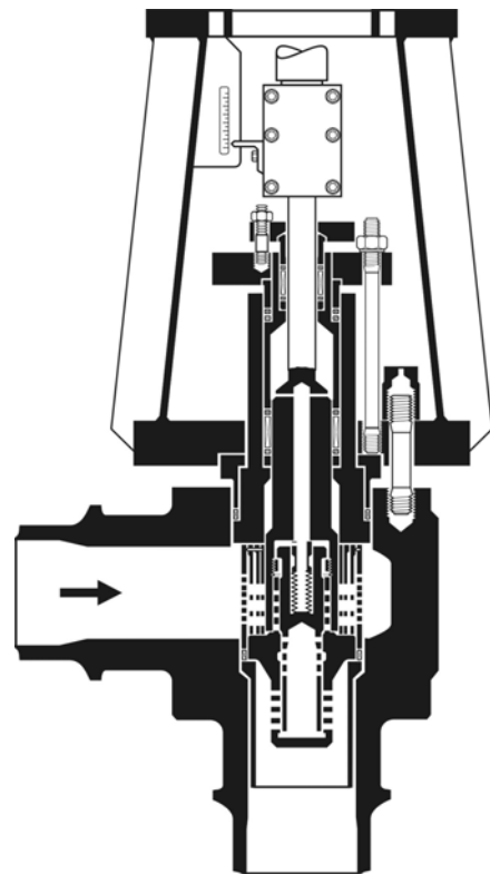
Control valve ZK 213-E.../... size 3 till 5, 6-stages
